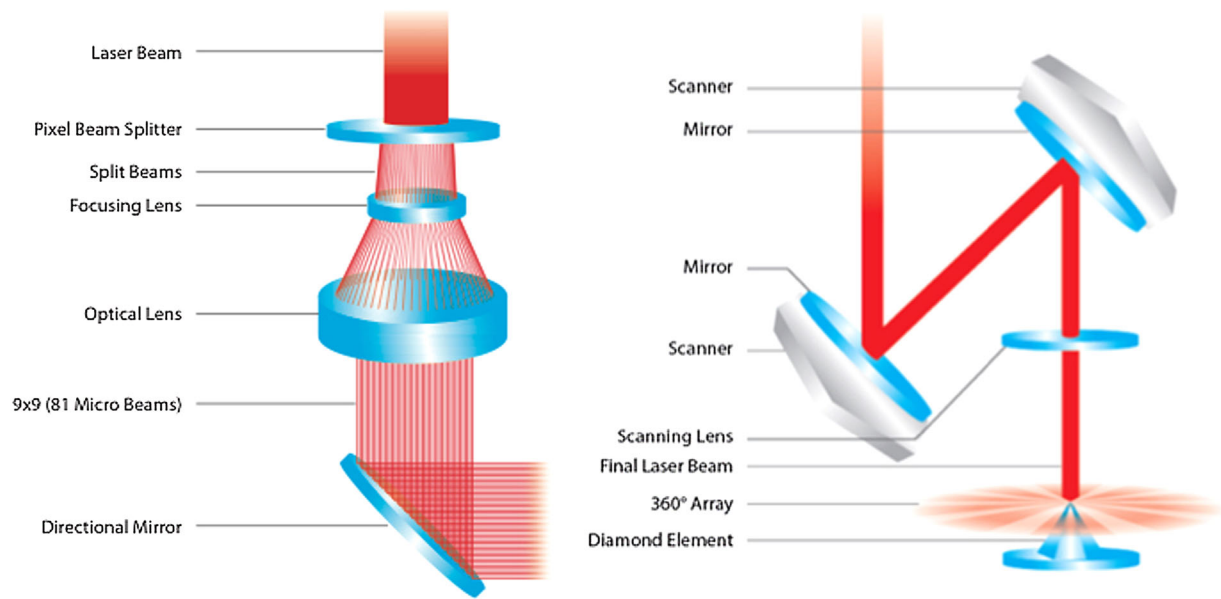
Fig. 5. (Left) Laser beam fractionated by holographic lens, printing 9 \times 9 (81 microbeams) on 10 \text{ mm}^2 . (Right) Laser beam delivered through computer controlled, two parallel mirrors and scanning lens. (Courtesy: Alma Lasers).
